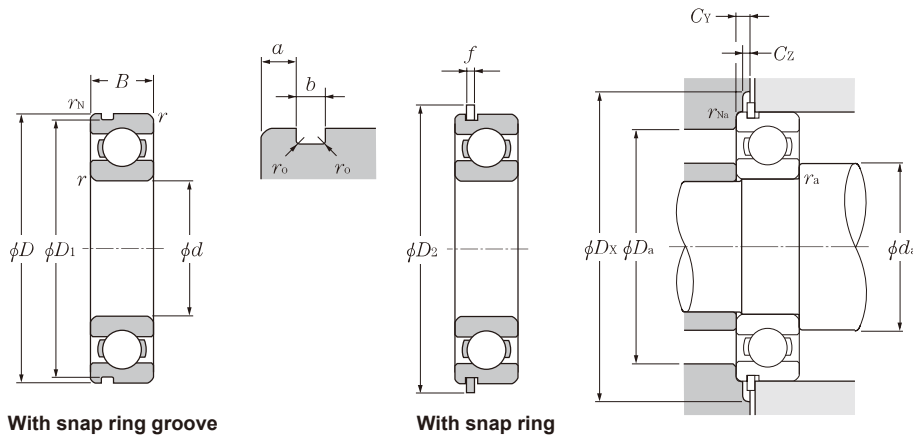
With snap ring groove
