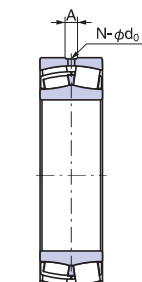
With oil holes / oil groove (W33)
