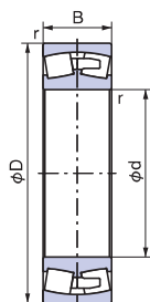
With machined brass cage
