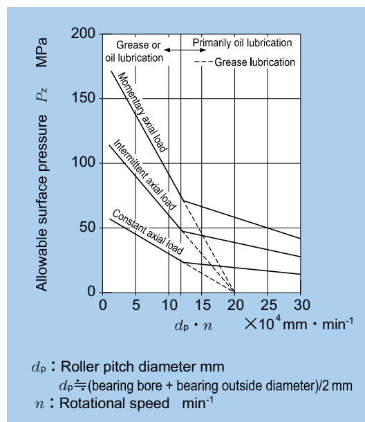
Fig. 1 Allowable surface pressure of rib
